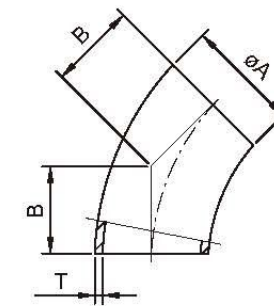
45° Short Elbow 2WK
